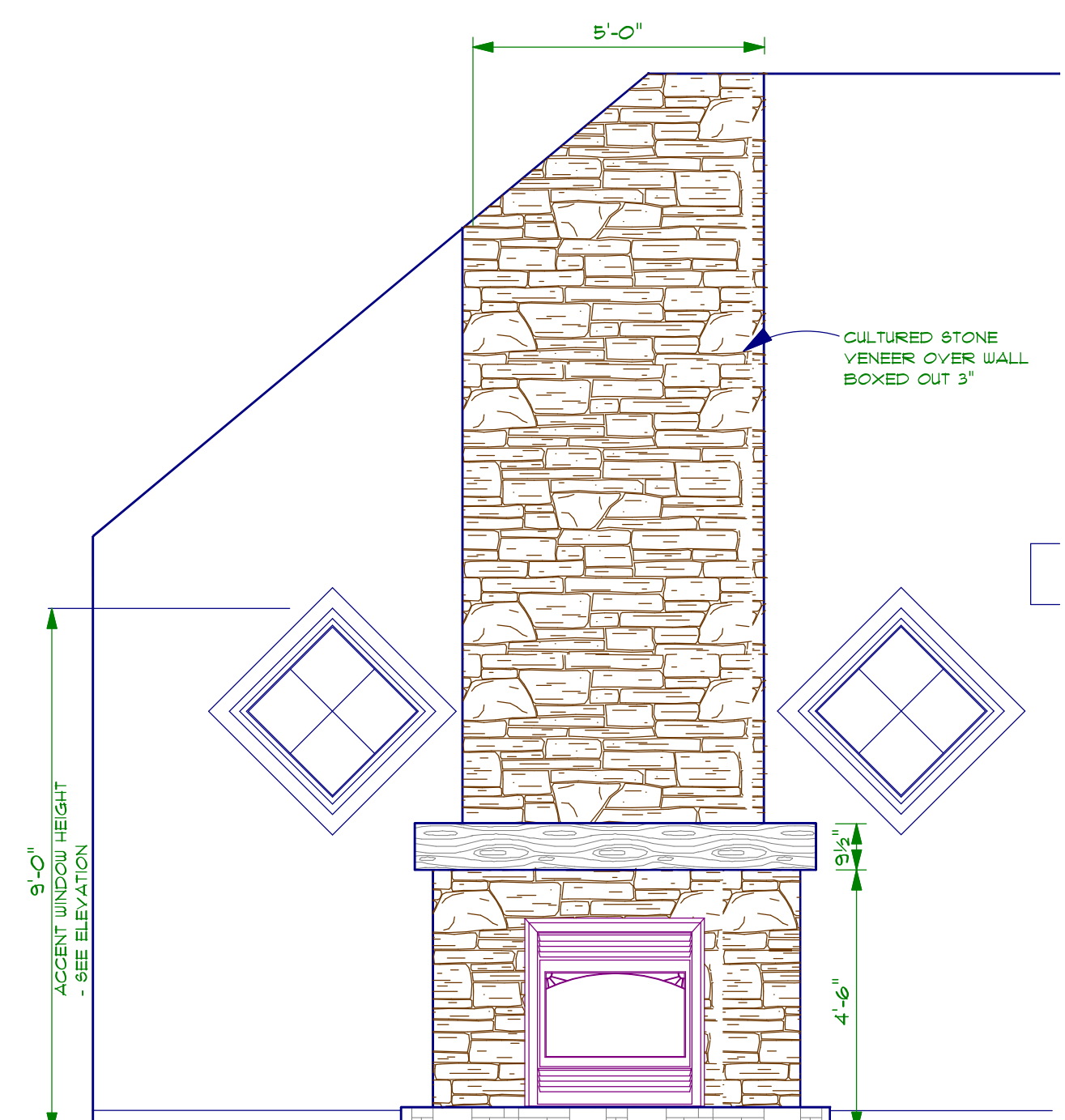
FIREPLACE ELEVATION - A 3/8" = 1'-0"
